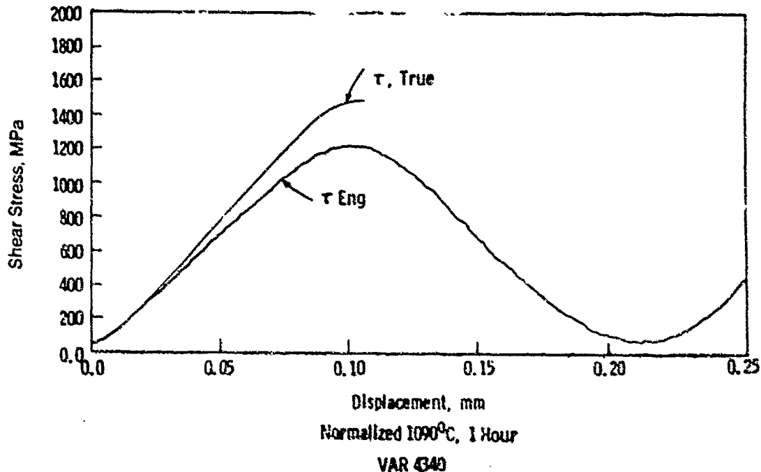
Figure 5. Typical engineering shear stress-displacement and true shear stress-displacement curves (true stress curve is only accurate up to the point of instability).
