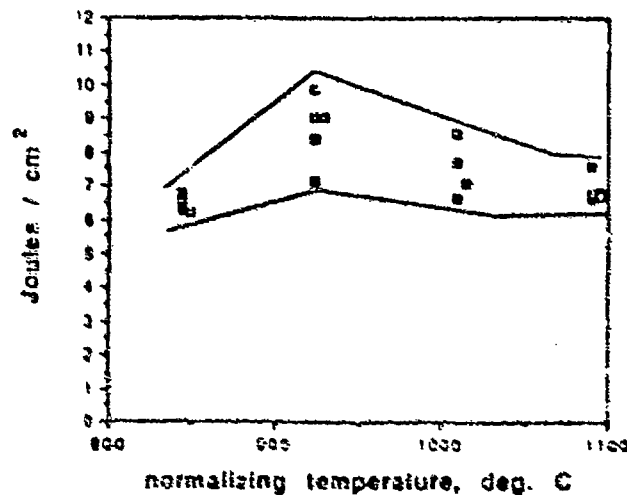
Figure 7. Energy absorbed to the point of instability per unit area sheared, E , versus normalizing temperature for a strain rate of \dot{\gamma} = 10^3\ \text{s}^{-1} .
