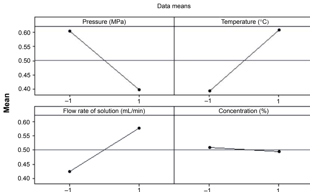
Figure 5 Main effects plot for particle size.
