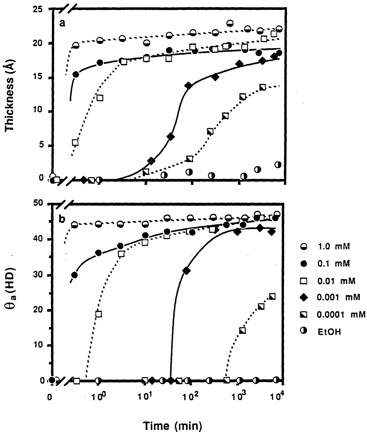
Figure 9. Kinetics of adsorption of octadecanethiol from ethanol as a function of concentration: (a) ellipsometric thickness (b) advancing contact angle of hexadecane (HD). EtOH ( \circ ) indicates pure ethanol containing no thiol.
