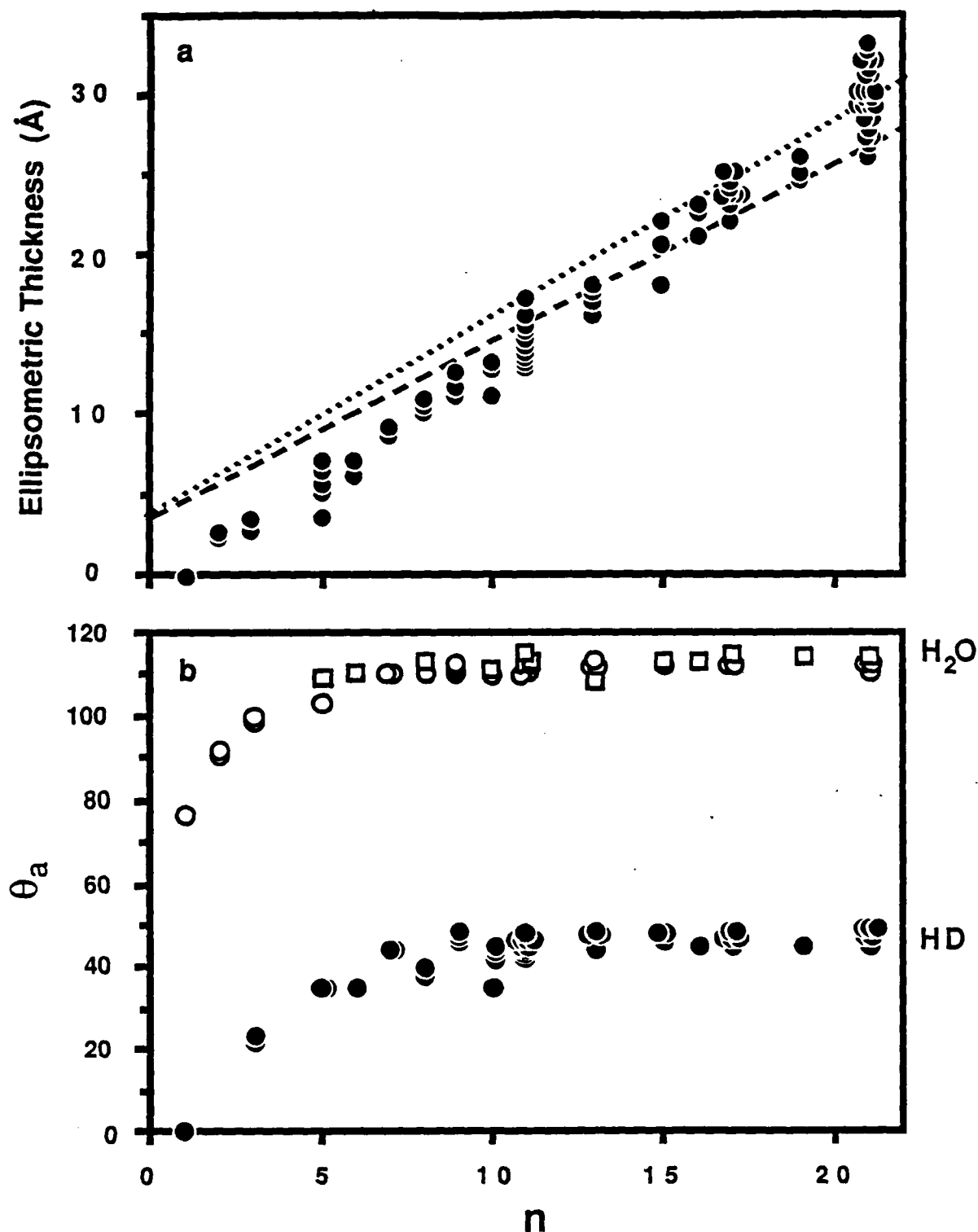
Figure 1. Monolayers of n-alkanethiols, \text{CH}_3(\text{CH}_2)_n\text{SH} , on gold. (a) Ellipsometric thickness. The dotted (dashed) line represents the thickness expected theoretically for a close-packed monolayer oriented normal (tilted 30° from the normal) to the surface. (b) Advancing contact angles: (●) hexadecane, (○) water, Method A, (□) water, Method B.
