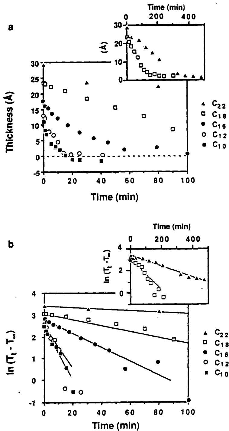
Figure 13. Thermal desorption of monolayers of thiols on gold in contact with hexadecane at 83 °C. (▲) docosanethiol, (◻) octadecanethiol, (●) hexadecanethiol, (○) dodecanethiol, (■) decanethiol. (a) Ellipsometric thickness; inset shows complete desorption profiles for the two longest chain thiols. (b) First-order plot of the corrected thicknesses against time. T_t - T_\infty represents the difference in ellipsometric thickness between time t and long times. Solid lines are linear fits to data points with T_t - T_\infty > 3 Å.
