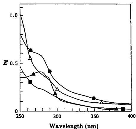
Fig. 4. Effect of reduction with sodium borohydride on: △, N' -formylkynurenine (0.03 mg/ml) in water; ▲, photo-oxidized tryptophan (0.03 mg/ml) in 0.03M-potassium phosphate, pH 7; ■, photo-oxidized lysozyme (0.4 mg/ml) in 6M-guanidinium chloride; ●, photo-oxidized normal human lens proteins (0.4 mg/ml) in 6M-guanidinium chloride.
