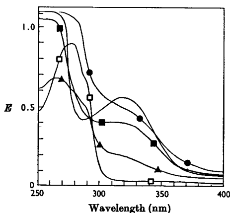
Fig. 2. Absorption spectrum of photo-oxidized substrates compared with that of N' -formylkynurenine and of lysozyme. —, N' -Formylkynurenine (0.03 mg/ml) in water, neutral; ▲, tryptophan photo-oxidized in sunlight (0.03 mg/ml) in water, neutral; ■, lysozyme photo-oxidized in sunlight (0.3 mg/ml) in 6M-guanidinium chloride; ●, normal human lens proteins photo-oxidized in sunlight (0.4 mg/ml) in 6M-guanidinium chloride; □, lysozyme, kept in dark (0.3 mg/ml) in 6M-guanidinium chloride.
