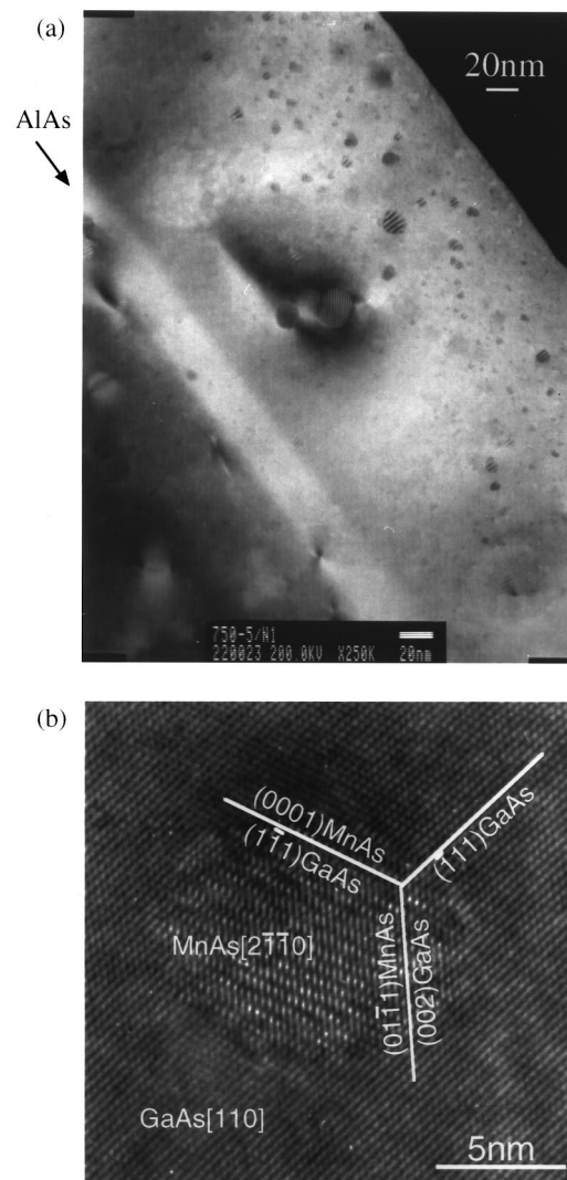
FIG. 1. (a) Cross sectional TEM image of LT-GaAs:Mn annealed at 750 °C (5 s) ( [Mn] = 1 \cdot 10^{16} cm -2 ). (b) High resolution TEM image of a single MnAs crystallite in LT-GaAs:Mn annealed at 750 °C (5 s) ( [Mn] = 1 \cdot 10^{16} cm -2 ).
