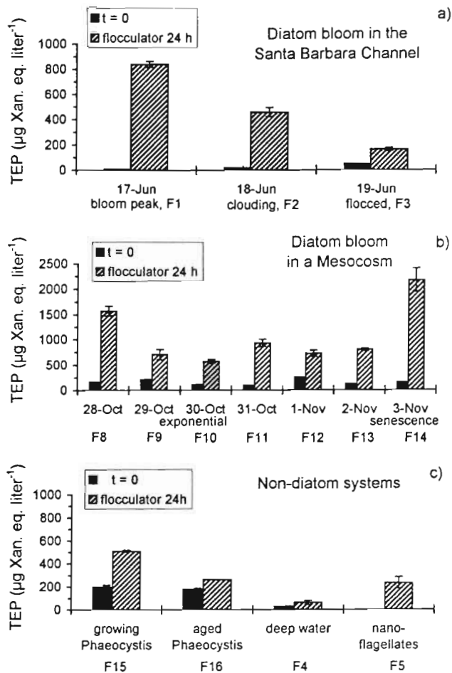
Fig. 1. Results of flocculator experiments. (a) diatom bloom in the Santa Barbara Channel, (b) diatom bloom in a mesocosm and (c) non-diatom systems. In each experiment concentration of TEP was measured in 0.2 \mu\text{m} filtered seawater initially ( t = 0 ) and after 24 h incubation in a flocculator (flocculator 24 h). Error bars are standard deviations of replicate TEP measurements (analytical replicates). Note change of scale
