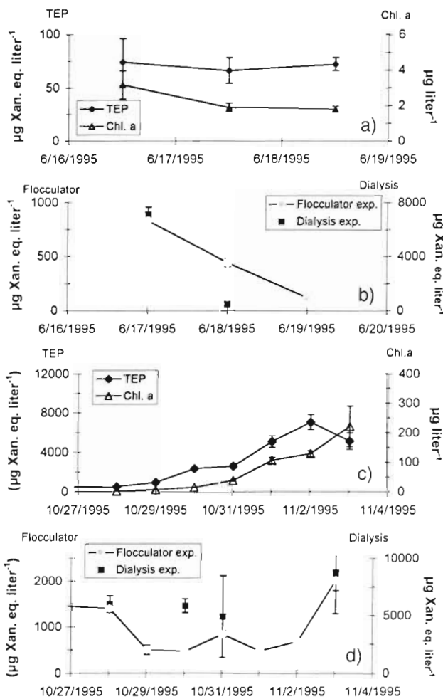
Fig. 3. (a,c) Ambient TEP and chl a concentration and (b,d) production of TEP in flocculator experiments (estimate of precursor concentration) and in dialysis experiments (relative estimate of precursor concentration + release rate) during (a,b) the diatom bloom in the Santa Barbara Channel and (c,d) the mesocosm bloom
