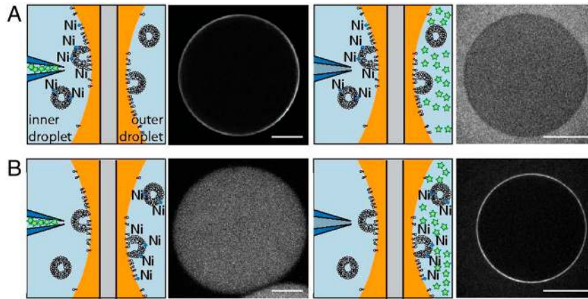
Fig. 2. GUVs with asymmetric lipid composition can be formed by controlling the SUV content of each reservoir. (A) SUVs containing Ni-chelating lipids were incubated in the droplet nearest the inkjet (inner droplet). His-GFP (green star) was either encapsulated in a GUV by microfluidic jetting (Left), or added to the outer droplet (Right), and the distribution of His-GFP was observed by confocal microscopy. (B) SUVs containing Ni-chelating lipids were incubated in the droplet furthest from the inkjet (outer droplet). His-GFP was either encapsulated in a GUV by microfluidic jetting (Left), or added to the outer droplet after vesicle formation (Right). All scale bars, 50 \mu\text{m} .
