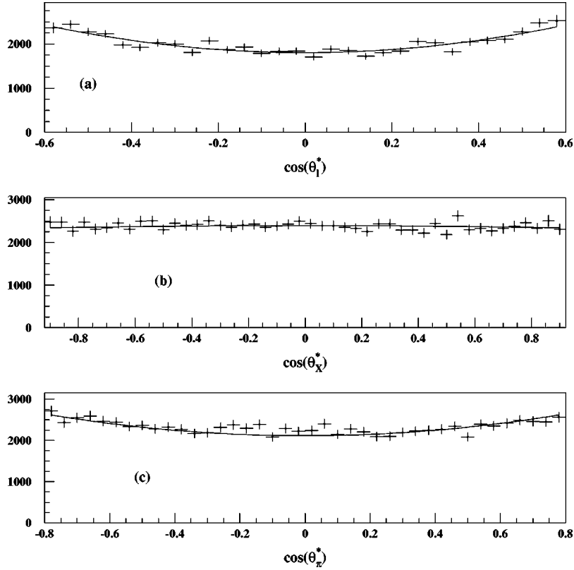
FIG. 5. Simultaneous fits ( \chi^2 ) to three 1D histograms of (a) \cos \theta_\mu^* , (b) \cos \theta_\chi^* , and (c) \cos \theta_\pi^* using Eqs. (3), (1), and (2), respectively. The phase shifts used are \delta_0^0 = 45^\circ and \delta_2^0 = 0^\circ .
