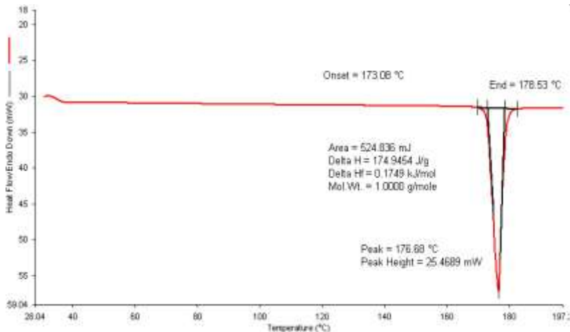
Figure 10: DSC Thermogram of Nifedipine API
