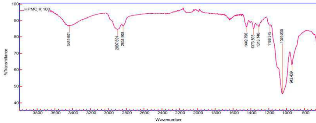
Figure 4 : FT-IR spectroscopy of HPMC K100
