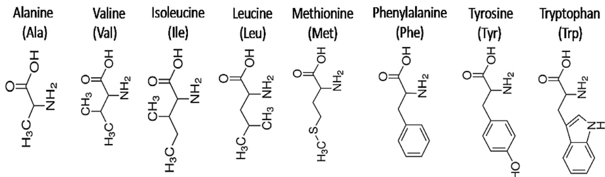
Fig. 1. Hydrophobic \alpha -amino acids tested in this work.
