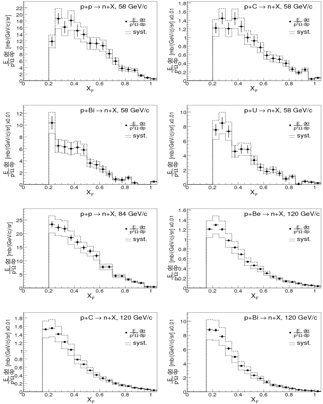
FIGURE 18. Lorentz-invariant cross-sections as a function of x_F for producing neutrons with momentum greater than threshold within the solid angle of the calorimeter.
