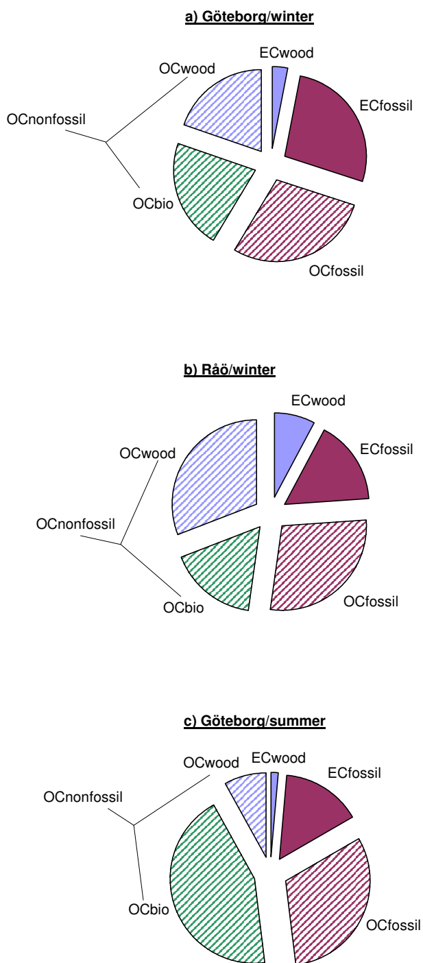
Fig. 6. Relative contributions of EC_{\text{fossil}} , EC_{\text{wood}} , OC_{\text{fossil}} , and OC_{\text{nonfossil}} (differentiated into OC_{\text{wood}} and OC_{\text{biogenic}} ) to TC for (a) urban site Göteborg/winter, (b) rural site Råö/winter, and (c) urban site Göteborg/summer.
