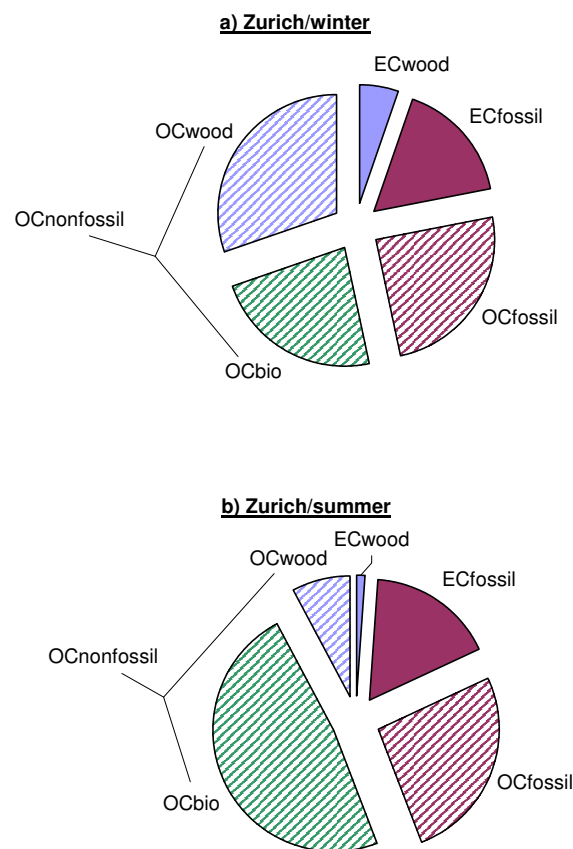
Fig. 7. Relative contributions of EC_{\text{fossil}} , EC_{\text{wood}} , OC_{\text{fossil}} , and OC_{\text{nonfossil}} (differentiated into OC_{\text{wood}} and OC_{\text{biogenic}} ) to TC according to Szidat et al. (2006) for (a) Zurich/winter (February 2003), (b) Zurich/summer (August 2002).
