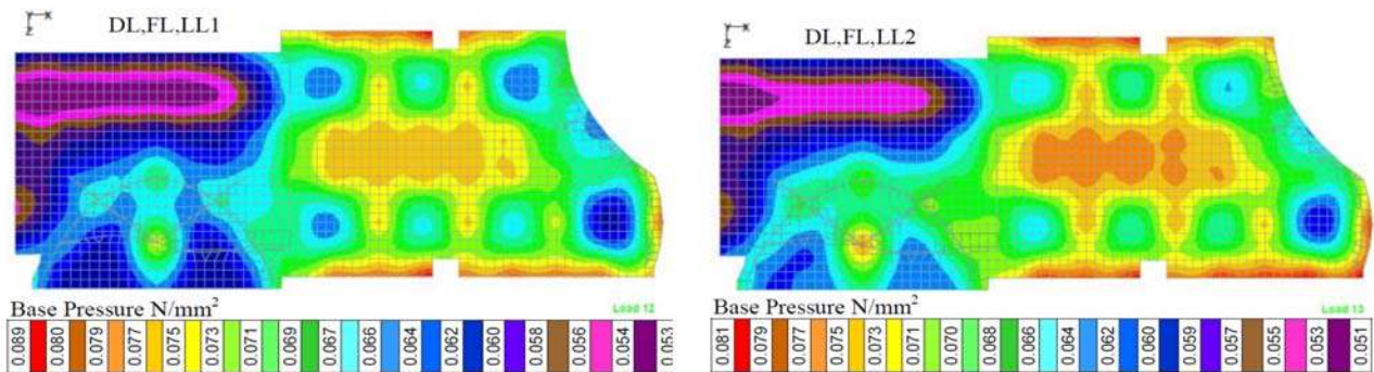
Fig. 8 Base pressure contour for Basra University (Case 3 and Case 4).
