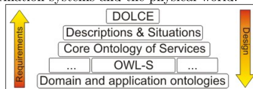
Figure 1: Ontology Stack.
