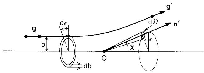
Fig. 7.2 Scattering from a collision center.
