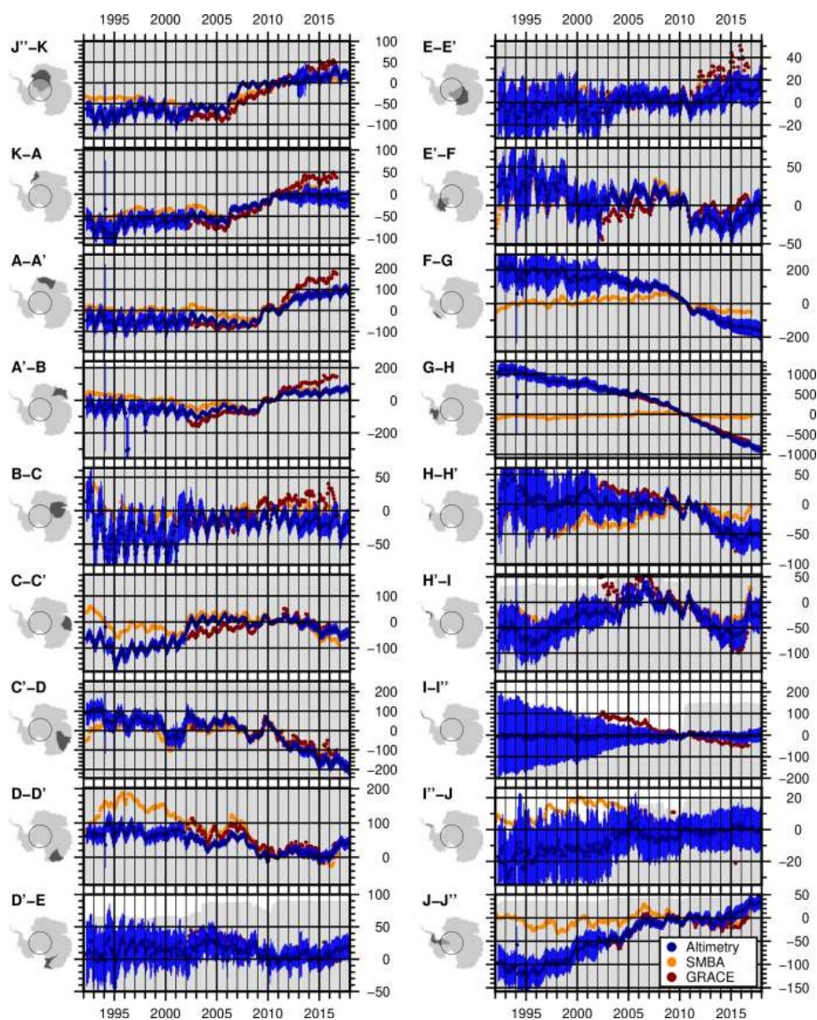
Figure 12. Mass change ( \Delta M [Gt]) of the individual drainage basins north of 81.5^\circ\text{S} from our combined altimetric time series (blue), GRACE (red) and SMBA (orange). The error bars show the uncertainty estimate \sigma_\Sigma of the altimetry data according to Sect. S6.2. The gray color in the background displays the fraction of the area covered by altimetry (the top of each panel means 100 %).
