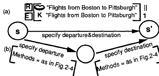
Figure 5: CARE and goal refinement.
