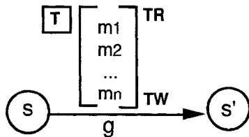
Figure 1: A notation for expressing CARE properties.
