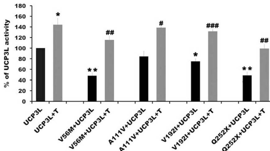
Figure 4 Effects of telmisartan treatment on palmitate oxidation activity of wt and mutant UCP3 proteins. Oxidation of ^3\text{H} -labeled palmitate in HEK293 cells expressing either UCP3L isoform or UCP3L and mutant UCP3 proteins in equal amounts (V56M/UCP3L, A111V/UCP3L, V192I/UCP3L and Q252X/UCP3L), in the absence (black bars) or presence (gray bars; +T) of telmisartan treatment. Data represent the means \pm s.d. of four different experiments reported as a percentage of the value obtained for UCP3L-expressing cells in the absence of telmisartan treatment (UCP3L black bar) to which we assigned an arbitrary value of 100%. * P < 0.05 and ** P < 0.005 vs UCP3L; # P < 0.05 , ## P < 0.005 and ### P < 0.001 vs corresponding black bar (-T).
