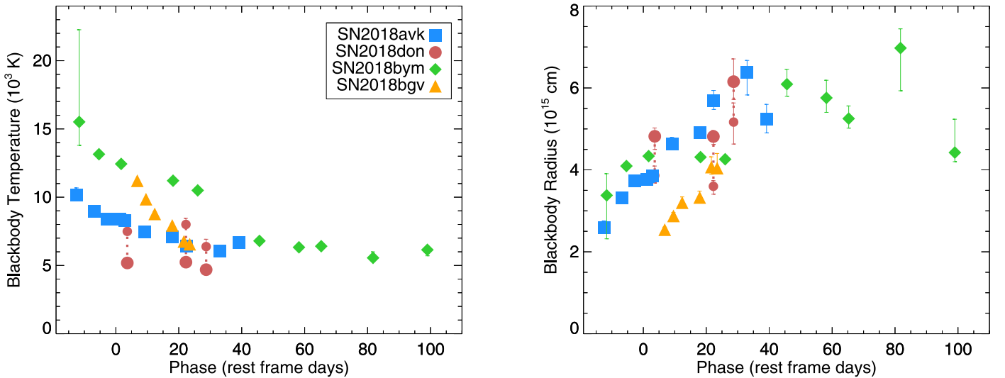
Figure 9. Derived blackbody temperatures (left) and radii (right) from fitting a Planck function to photometry epochs with at least three filters available. The smaller points for SN 2018don show the inferred values if assuming host galaxy extinction according to E(B - V) = 0.4 mag.
