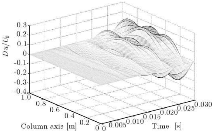
Fig. 17. No controlled-controlled normalised displacement difference vs. time and column axis for the first resonance
