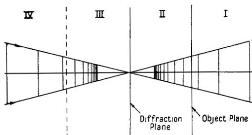
Figure 4. Distribution of Fourier image planes for a divergent pencil incident on the object
