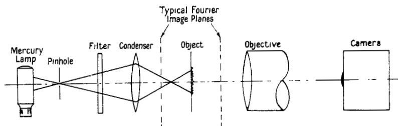
Figure 5. Experimental arrangement.
