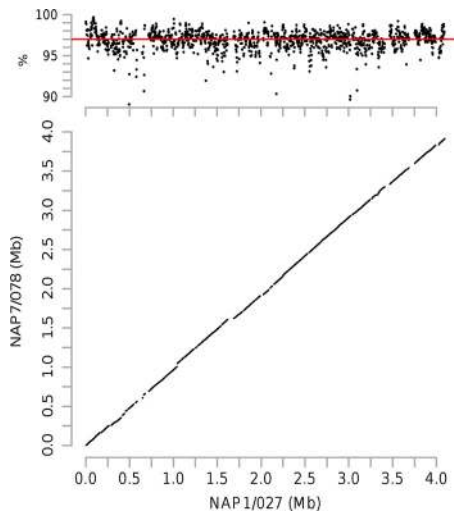
FIG. 1. Percent identity plot (top) and dot plot (bottom) depicting the whole-genome pairwise alignments of a NAP1 isolate (QCD-66c26) and a NAP7 isolate (QCD-23m63). The dot plot in the bottom panel depicts the colinearity of the two genomes, and the percent identity plot in the upper panel depicts the levels of nucleotide-level similarity of the two genomes (the red line indicates average percent identity).
