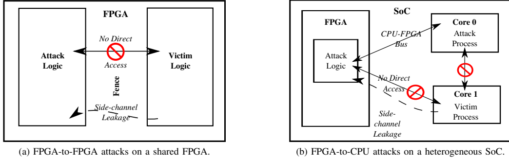
Fig. 1. Threat models.
