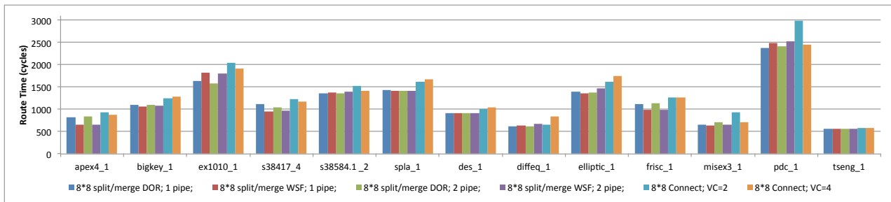
Fig. 7: Cycle Comparison between CONNECT and Split-Merge PS NoC on Bellman Ford Application Traffic on 8 \times 8 Mesh
