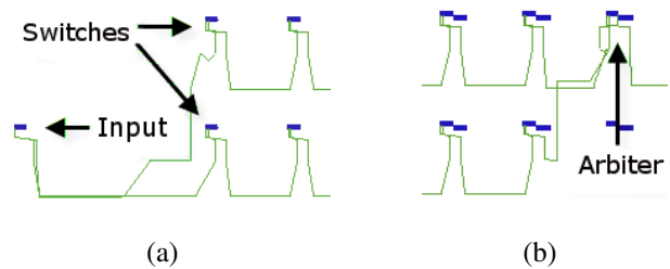
Fig. 8. Routing and placement of the PUF (a) first segment (b) last segment.
