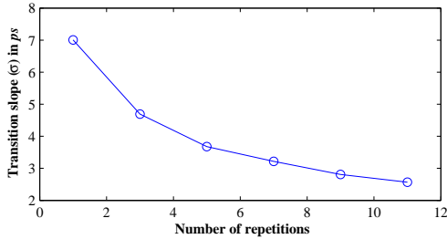
Fig. 14. The sharpness ( \sigma ) of the transition slope versus the number of repetitions for majority voting.
