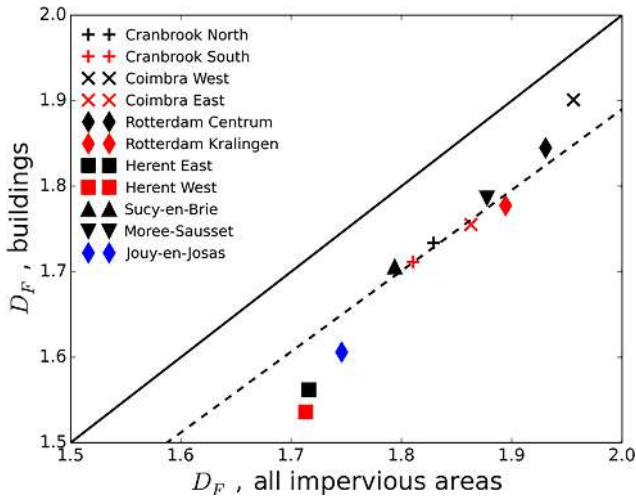
Figure 11. Empirical relation between the fractal dimensions of the total impervious area and of buildings only. The continuous line indicates the first bisector, while dotted line is given by D_{F,build} = 0.945 D_{F,all} .
