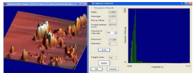
Figure 7. AFM images of surface roughness without carbon nano tube based nanofluids, speed = 1500 Rpm, Ra = 0.4897 µm.
