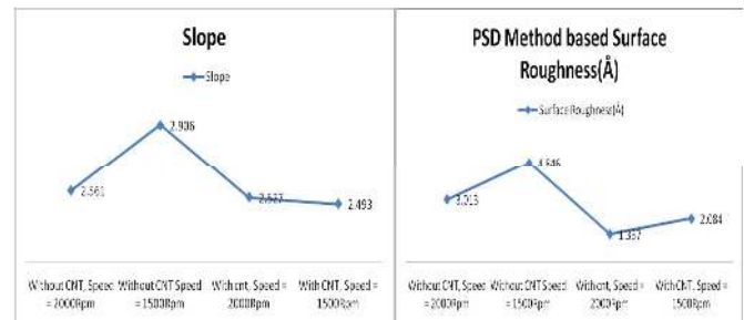
Figure 14. Slope and PSD method based surface roughness comparison for different machining conditions.
