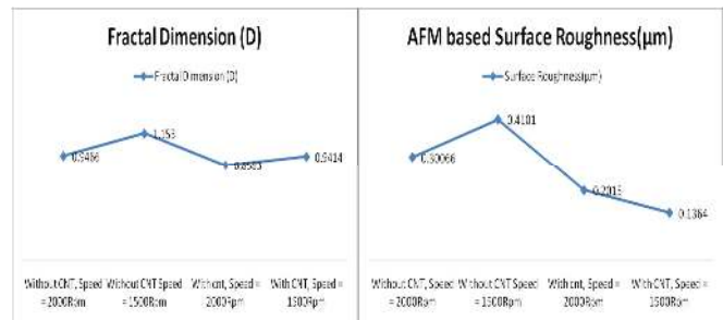
Figure 19. Fractal dimension and surface roughness analysis for different machining conditions.
