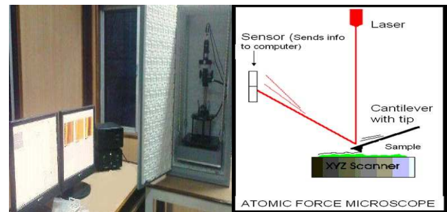
Figure 4. Measurement setup (left) and schematic diagram (right) of AFM.
