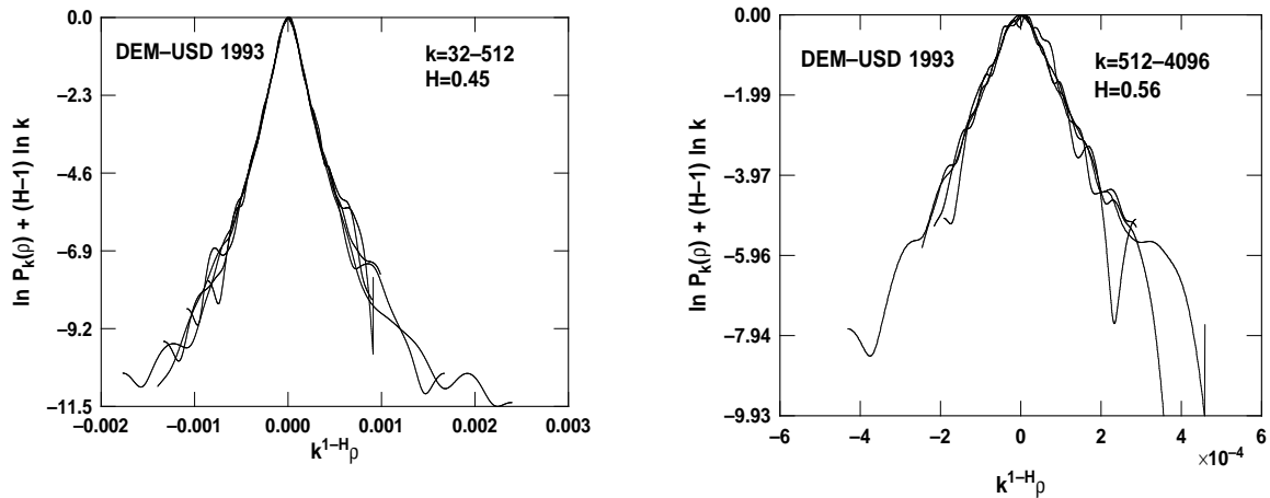
Figure 5: For the DEM-USD price record there is cross-over in the scaling behavior of the mean absolute lag- k return. Left ) For time scales of 32-512 quotes, one finds a high degree of distributional self-similarity, with the basic distribution Q shown in the left plot. The right plot show the basic distribution for the longer time scales. One observes that not only the exponent H changes when going from the short time scaling regime to the long time one: Also the shape of the basic distribution changes.
