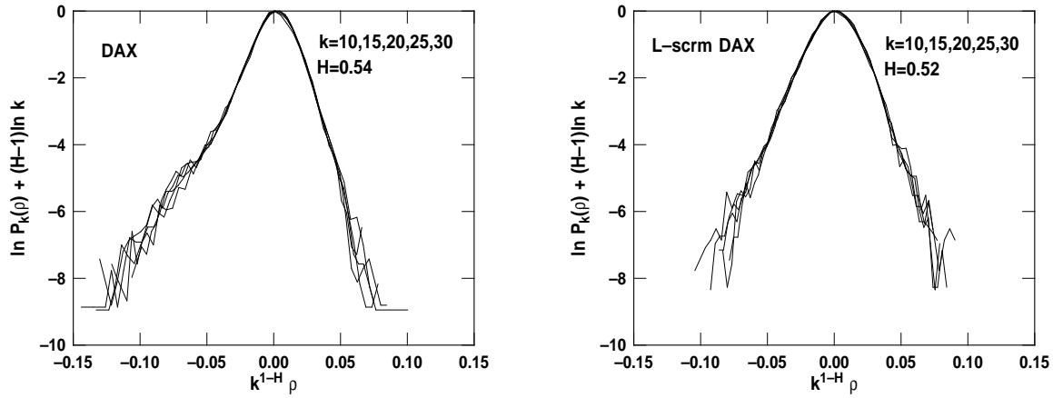
Figure 4: Left ) The basic distribution Q for the DAX stocks in the period November 3, 1986 till August 4, 1993. The rescaling rule Equation 3 is used with the self-similarity exponent H = 0.54 . Right ) The same analysis, however, with DAX stocks in which the daily returns have been scrambled to get rid of correlations. The change in shape shows that correlations between the daily returns do play a role in the price formation. The tails are a bit shorter, because a shorter period has been used – November 3, 1986 till September 7, 1992.
