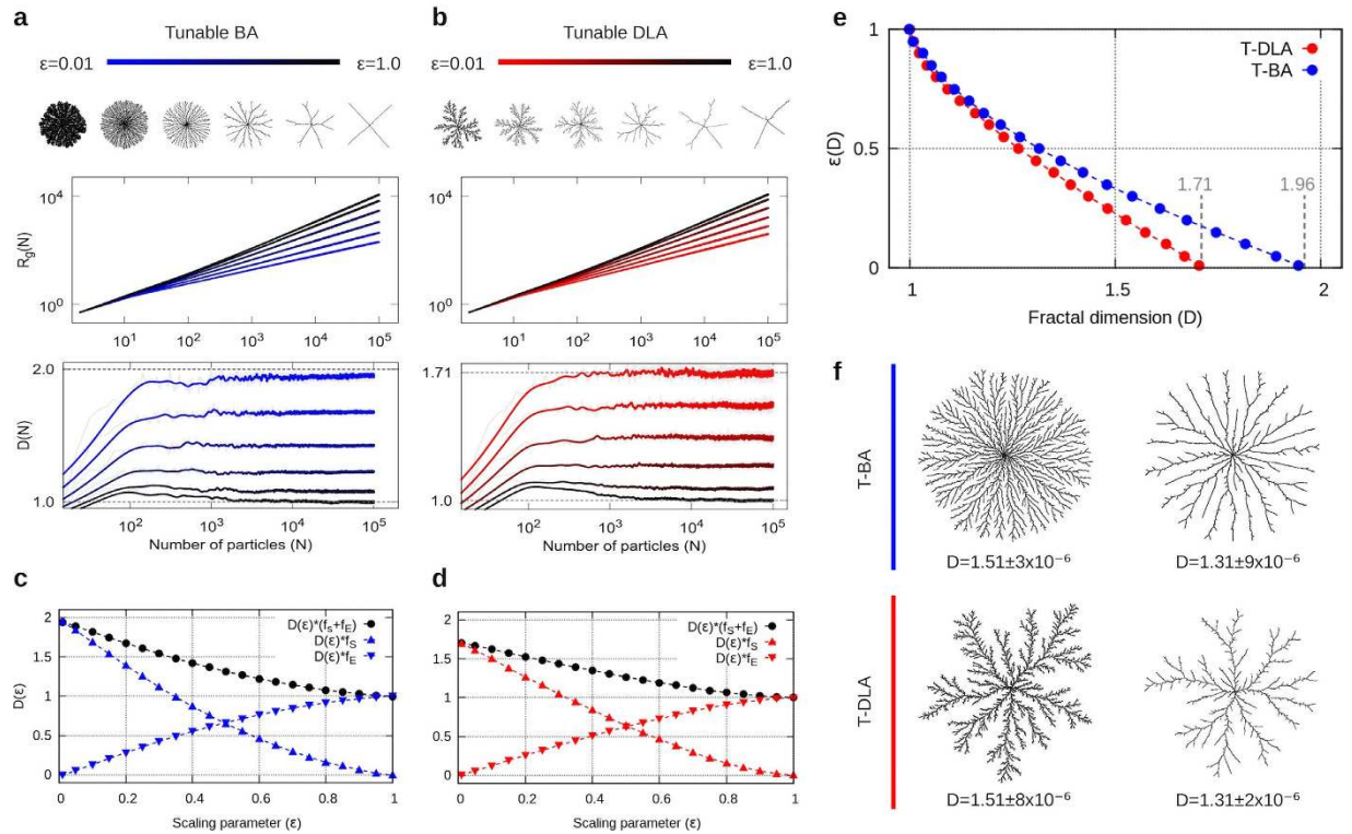
Figure 4. Tunable aggregates. (a,b) Log-log plots for R_g(N) and lin-log for D(N) , for aggregates grown with specific values of \epsilon in [0.01, 1] , for BA (blue) and DLA (red) up to N = 10^5 particles. Notice how the multiscaling behavior gives way to a single well-defined fractal dimension D = D(\epsilon) . One can also appreciate the difference in the morphology of these monofractal-aggregates with respect to \epsilon at the top. (c,d) Plots of the specific entropic [D(\epsilon)f_s] and energetic [D(\epsilon)f_E] contributions to the clusters' fractal dimension D(\epsilon) for BA and DLA as above. (e) Plots of \epsilon vs. D for aggregates based on DLA and BA. These numerically obtained curves can be used to grow clusters with any prescribed D . (f) BA- and DLA-based clusters with the same fractal dimension, D = 1.51 and 1.31 , grown with a very high precision in D .
