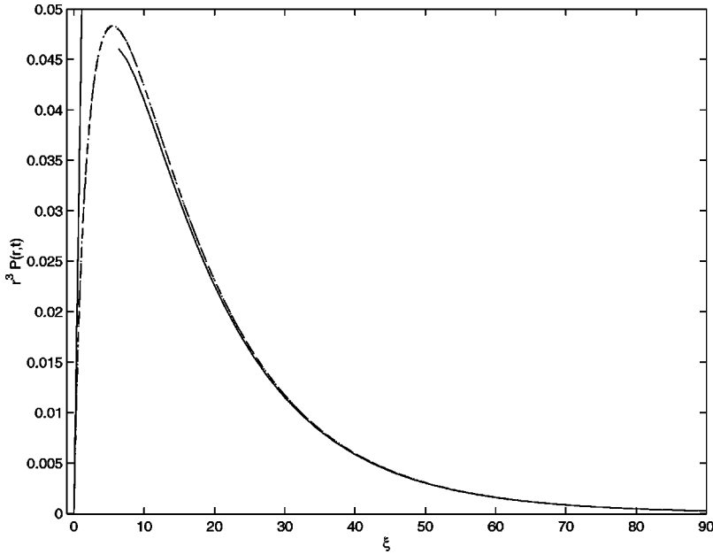
FIG. 3. Scaling behavior of P(r,t) for \alpha = 1/2 and d = 3 . We show r^3 P(r,t) vs \xi = r^2/t^\alpha for times t = 0.02 (dotted line), t = 2 (dash dotted line), and t = 200 (dashed line). Due to the exact scaling of the solution one cannot distinguish between the three curves in the figure. Also shown (solid curves) are the two asymptotic behaviors valid for small and large values of the scaling variable \xi . For \xi \gg 1 we used Eq. (34), and for \xi \ll 1 we used the leading term in the expansion [Eq. (35)].
