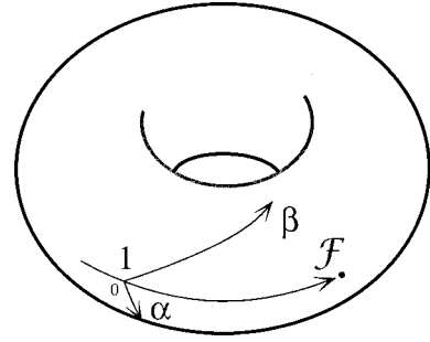
Fig. 2. Torus \mathcal{T}^2 of x - y -separable FT's \mathbf{F}_1^{\alpha,\beta} . The unit transform is at \mathbf{1} = \mathbf{F}_1^{0,0} , and the official FT is at \mathbf{F} = \mathbf{F}_1^{n_1,n_2} , with n_1, n_2 \equiv 1 \pmod{4} . The \alpha = \beta circle is composed of central FT's. For a given (\alpha_0, \beta_0) , the continuous powers (t\alpha_0, t\beta_0) may or may not pass through the official transform.
