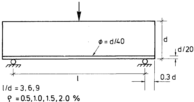
Fig 5.3 (8) Geometrical shapes of beams. \rho =percentage of re.
