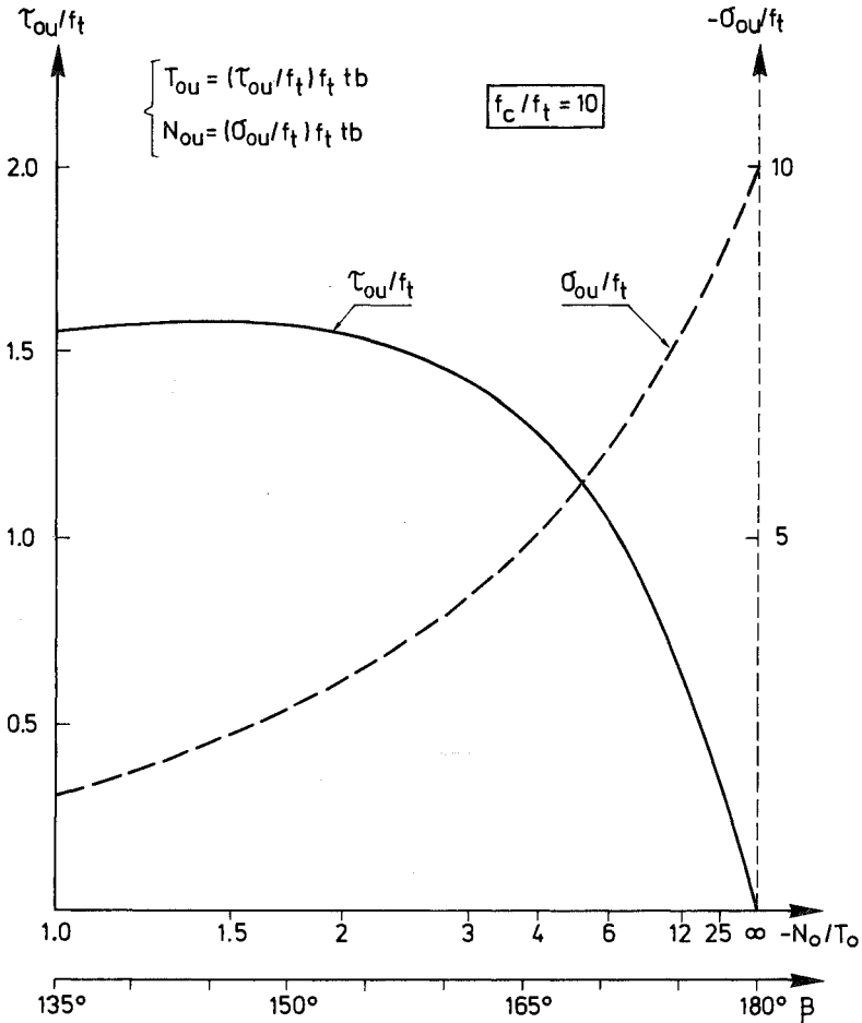
Fig 5.3 (6) a) \tau_{ou}/f_t and -\sigma_{ou}/f_t versus -N_o/T_o and \beta .
