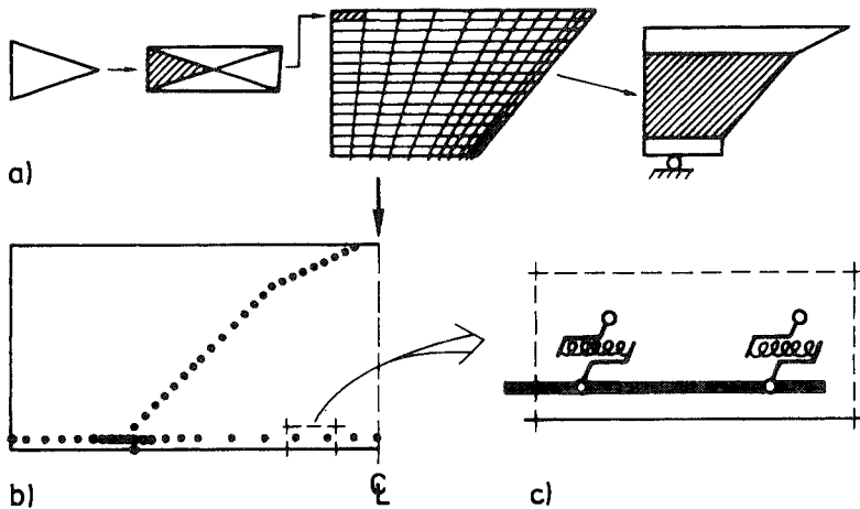
Fig 5.3 (2) a) Building up of a typical concrete block from constant strain elements. b) Nodes in assembled concrete blocks before start of node opening. c) Linkage of reinforcement bar elements to concrete by bond stress-slip elements.
