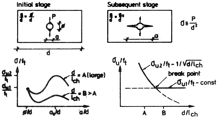
Fig 3.5 (2) Exemplification to possibility of abrupt break-points in a \sigma_u/f_t vs. d/l_{ch} curve.
