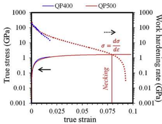
Fig. 6. True stress (solid lines) and work hardening rate (dotted lines) as a function of true strain of QP400 and QP500.
