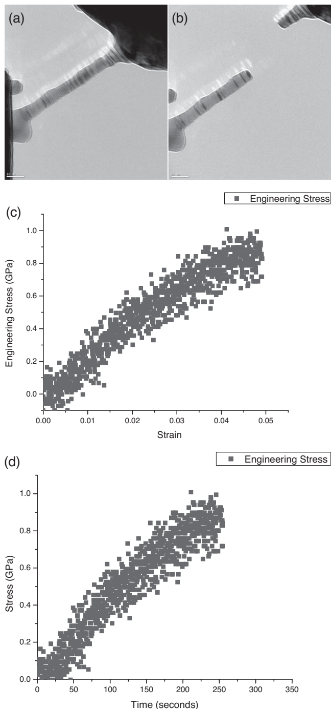
Figure 2. A typical brittle-like fracture of a long nanowire under tension with a low loading rate ( \sim 0.1 nm/s): a) initial state; b) after breaking (scale bar 10 nm); c) corresponding engineering stress-strain curve; d) engineering stress as a function of loading time.
