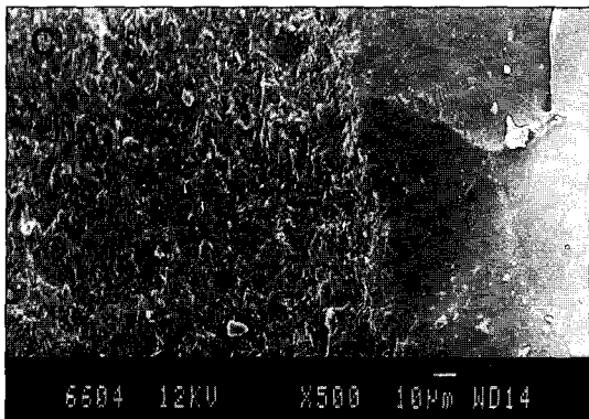
Fig. 6. SEM view of homogeneous structure of the core material and tight junction to the veneer porcelain : A, In-Ceram. B, Copy-milled In-Ceram. C, IPS Empress 2. (Original magnification × 500.)
