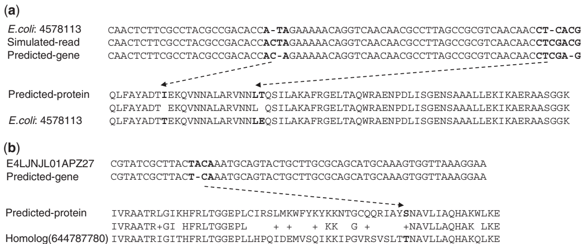
Figure 4. Examples of fragmented genes that contain frameshift sequencing errors: a gene predicted from a read simulated from the E. coli genome starting at position 4 578 113 (a), and a gene predicted from a metagenomic read from the TS28 dataset (b). The alignments of the nucleotide sequences are partially shown for clarity. The dotted lines connect the regions of nucleotides (with sequencing errors fixed) and the amino acid(s) that they encode. The alignment between the predicted protein from the metagenomic read and its homolog identified in IMG protein database is also shown.
