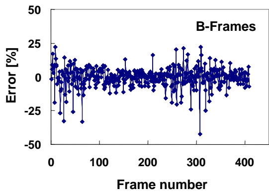
Fig. 7. Errors in B-frame workload prediction
