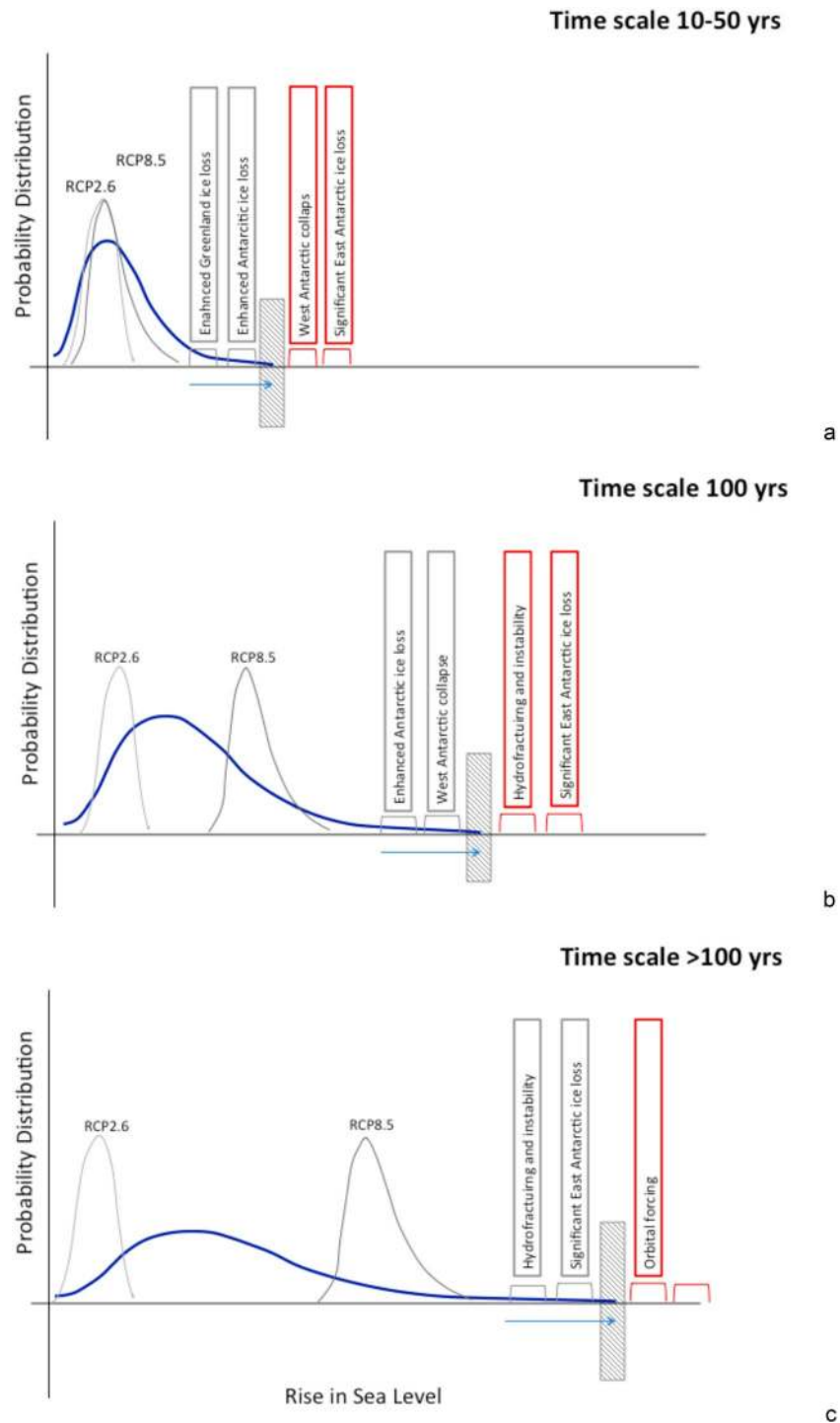
Figure 3. Concepts of sea level rise as a function of time scale. (a) Decadal to multidecadal time scale for which natural variability is a significant factor. (b) One hundred-year time scale equivalent to the 100-year projection discussed in fifth Assessment Report (Church et al., 2013). (c) Two hundred plus year time scale. The building blocks might shift from red to gray if the time scale of interest gets longer. The distinction between gray and red building blocks is lines of evidence vs physical implausibility as a function of time scale.
