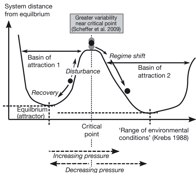
Fig. 4. The landscape metaphor for stability and regime shift (Holling 1973). The ball, representing ecosystem state, moves between valleys denoting different regimes, following disturbance (to the ball (Krebs 1988) or changes in the landscape (Scheffer et al. 2001). In the metaphor, stabilizing effects are likened to gravity. In mathematical terms, stability is the result of the system's tendency to move towards an attractor state, shown at the bottom of each basin
