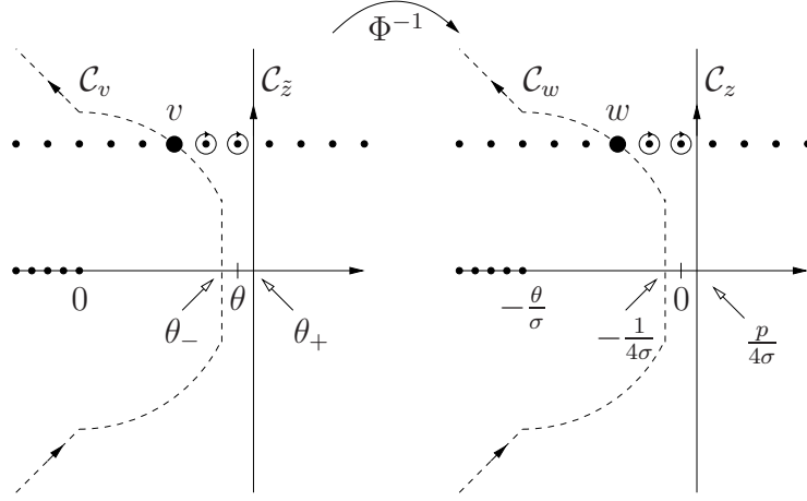
FIGURE 8. Left: Integration paths \mathcal{C}_v (dashed) and \mathcal{C}_z (the solid line plus circles at v+1, \dots, v+\ell ), where \theta_+ = \theta + p/4 and \theta_- = \theta - 1/4 , the small black dots are poles either of the sine or of the gamma function. Right: Integration paths after the change of variables \mathcal{C}_w (dashed) and \mathcal{C}_z (the solid line plus circles at w+1, \dots, w+\ell ), with p = p(w) \in \{1, 2\}
