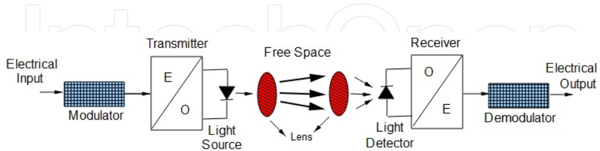
Figure 5. Block diagram of an optical wireless link showing the front end of an optical transmitter and receiver [7].
