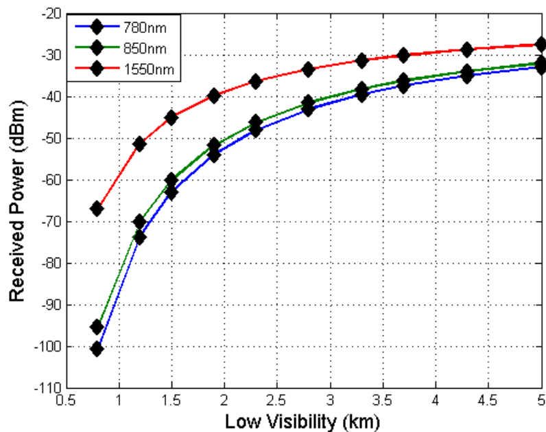
Figure 27. Received power (dBm) versus low visibility (km).
