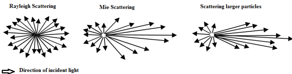
Figure 8. Patterns of Rayleigh, Mie and Non-selective scattering.
