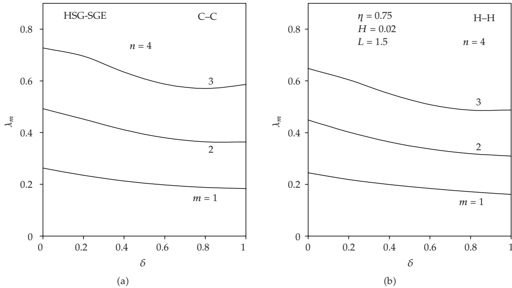
Figure 2: Variation of frequency parameter with relative layer thickness: linear variation in thickness of layers.
