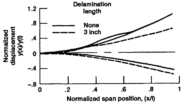
Figure 13.—Measured mode shapes: effect of delamination at interface 3.
