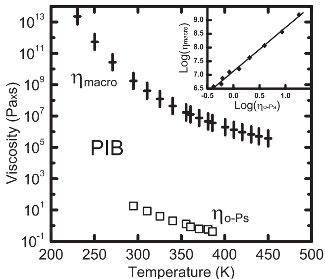
FIG. 4. Comparison of macroscopic ( t , \eta_{macro} ) and estimated nanoscopic viscosity ( \square , \eta_{o-Ps} ) of PIB. The macroscopic viscosity was calculated from a relation by Fox and Flory (Ref. 40). The lengths of the vertical bars used as symbols mark the variation of the calculated viscosity for different molecular weights (Ref. 41). The nanoscopic viscosity was estimated using the Navier-Stokes equation (see text). Inserted in top right corner is a log-log plot of the estimated correlation between \eta_{macro} and \eta_{o-Ps} which has been approximated by a straight line (Eq. (8)).
