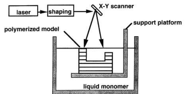
Fig. 1. Schematic of the 3D Systems' stereolithography apparatus (SLA) for fabrication of three-dimensional objects.
