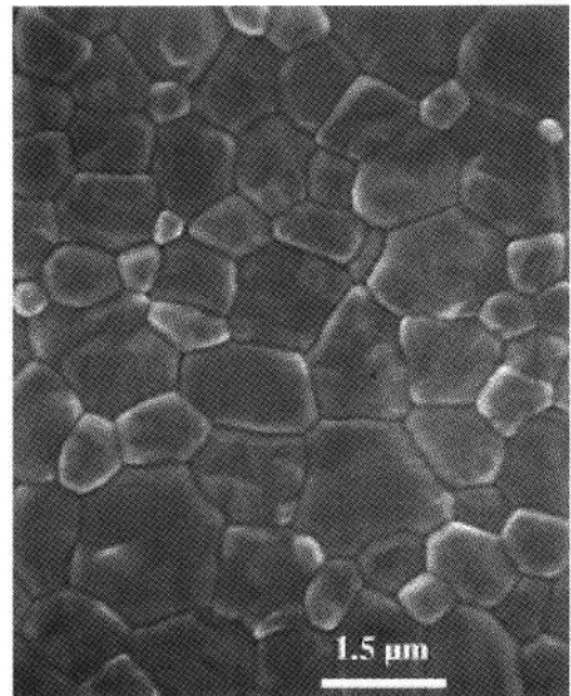
Fig. 10. Sintered alumina windowpane showing fully dense microstructure with grain sizes between 1 and 2 μm.
