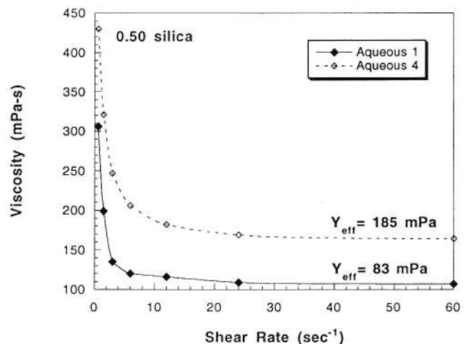
Fig. 5. Viscosity versus shear rate for 0.50 solids loading silica in two aqueous solutions, Aqueous 1 ( n = 1.382 ) and Aqueous 4 ( n = 1.418 ). Both suspensions have low yield point, Y_{\text{eff}} , values.
