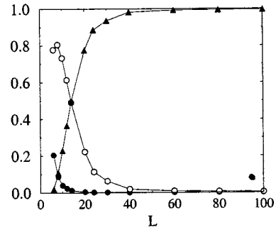
FIG. 7. Probability that the system reaches the ground state (dots), a frozen metastable state (circles), or a blinker state (triangles) as a function of the linear dimension. The number of realizations is \geq 10^4 for each system size. The lines are a guide for the eye.
