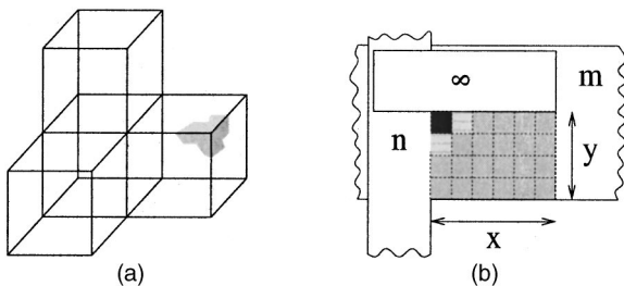
FIG. 6. (a) A three-arm star consisting of four cubic blocks of linear dimension L/2 in an L \times L \times L system with periodic boundary conditions. The other phase occupies the remainder of the volume. A convex corner (for free boundary conditions) is shown shaded. (b) Stochastic blinker on the cubic lattice. The shaded region of size x \times y \times (n - m) contains a fluctuating interface which can range between all spins up and all spins down.
