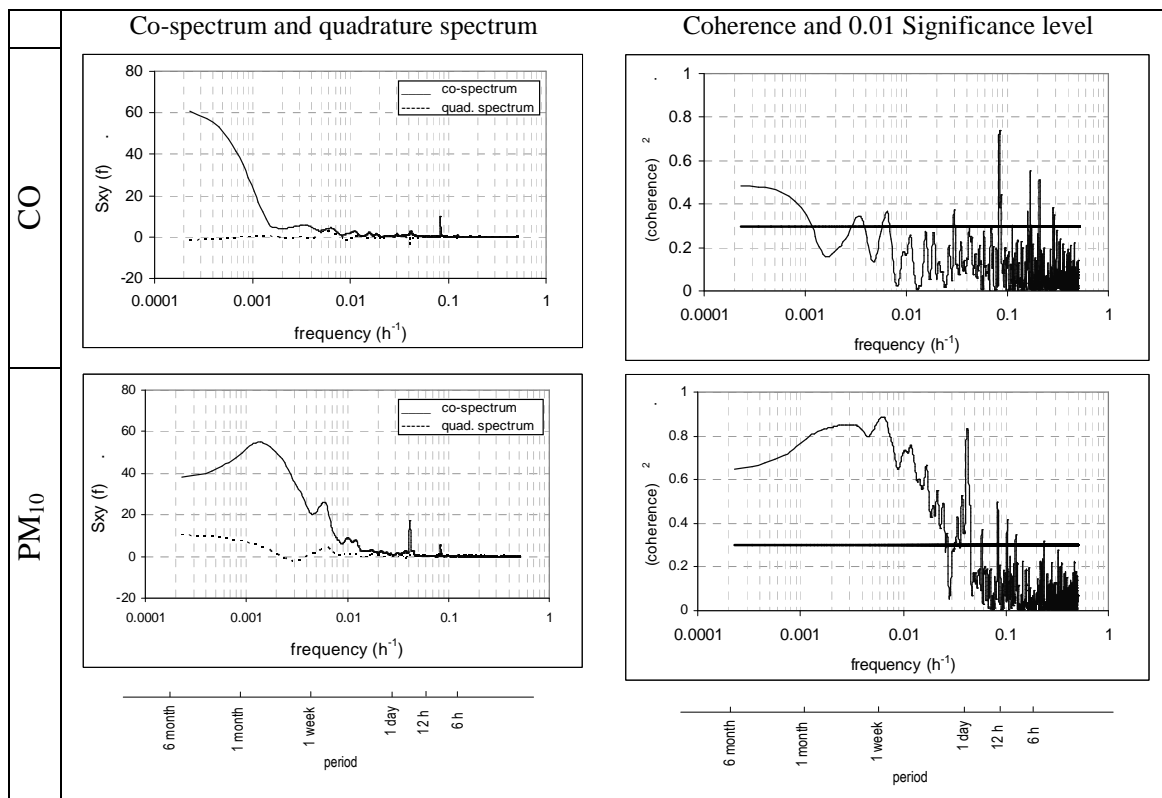
Figure 10. Co-spectrum, quadrature spectrum and coherency spectrum for CO and PM 10 concentrations: Antas urban station versus VNTelha suburban background station.
