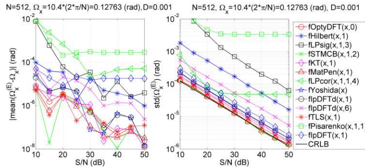
Fig. 5. Mean value and standard deviation of frequency estimation.
