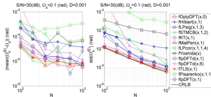
Fig. 8. Mean value and standard deviation of frequency estimation.
