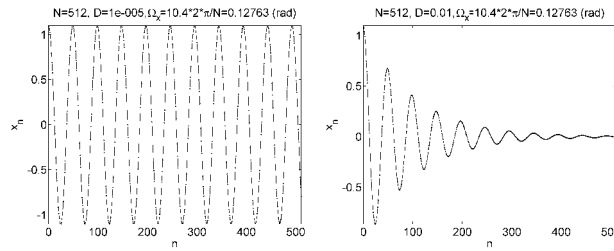
Fig. 1. Example model test signals.
