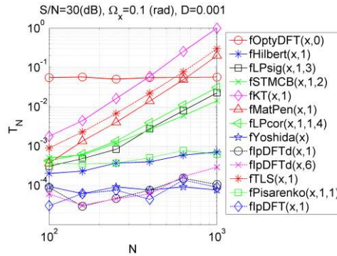
Fig. 11. Normalized computational time.
