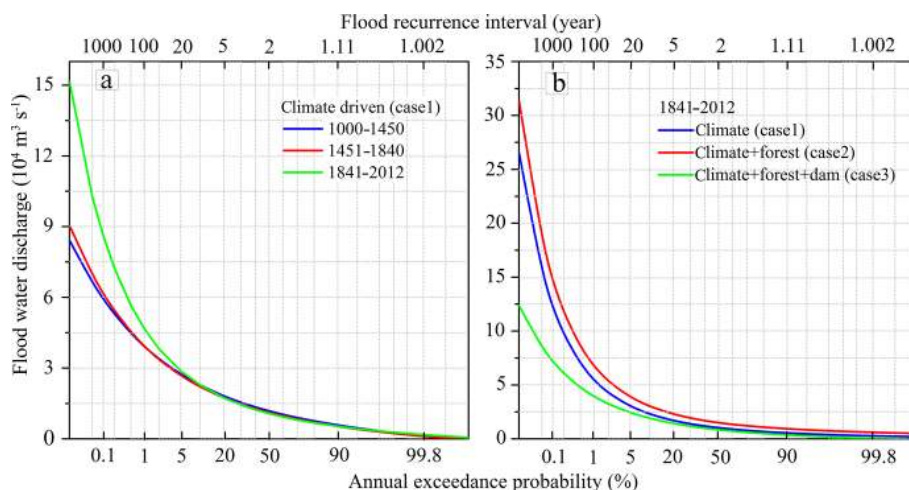
Figure 10. Frequency curves of annual maximum daily discharge for the Yalu River under different scenarios: (a) design floods estimated by three periods with different climatic characteristics, and the different effects of human activities in three periods were eliminated; (b) design floods estimated by dataset during 1841–2012 by setting three scenarios (climate, climate + forest cover, and climate + forest cover + dam).
