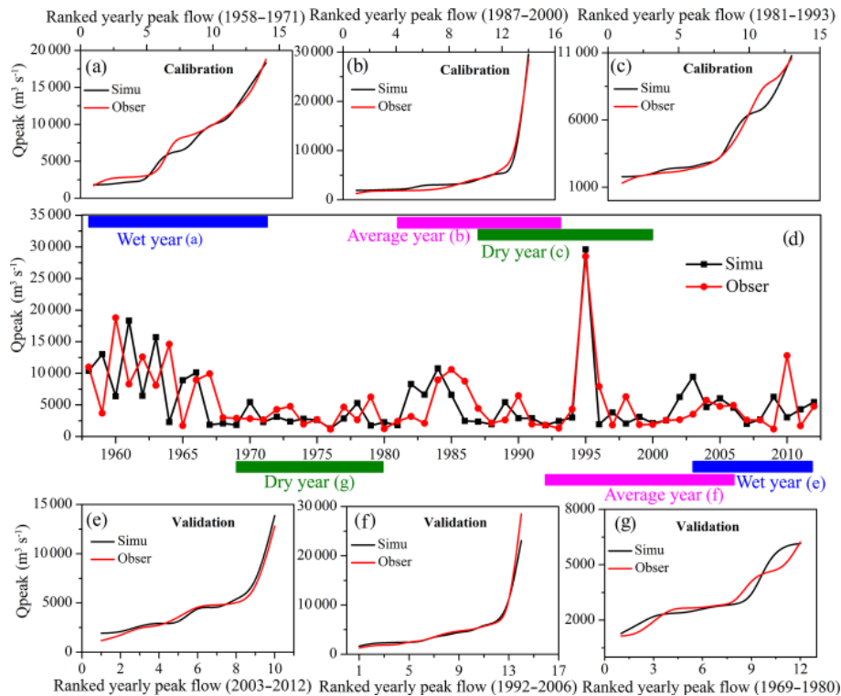
Figure 5. Comparisons of simulated and observed peak discharge of the Yalu River: (a–c) show ranked peak flows between the model simulations and observations for wet, average, and dry years during the calibration period, respectively; (e–g) show ranked peak flows between the model simulations and observations for wet, average, and dry years during the validation period, respectively; and (d) is the time-series comparison of simulated and observed daily peak flow during 1958–2012.
